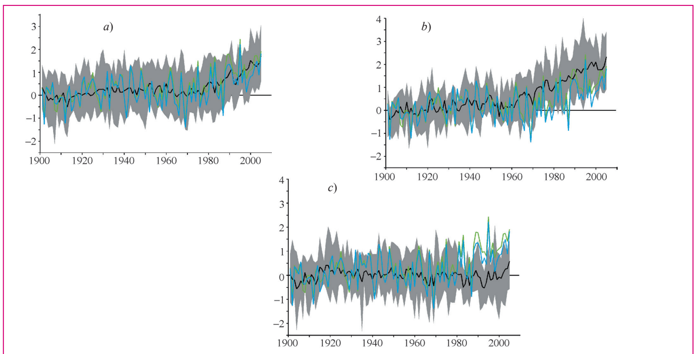
Fig. GS2.3. Anomalies of mean annual surface air temperature in Russia from observational data (green and blue curves) and CMIP5 ensemble means (black curve) with natural and anthropogenic forcings (a); major greenhouse gas (GHG) forcing only (b); natural forcings only (c). Anomalies are calculated relative to the 1901–1930 baseline period. Inter-ensemble spread is shown in grey.
